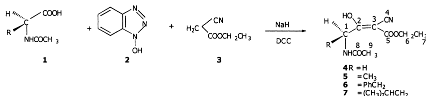
Scheme 1. Synthesis of compounds 4–7 .
